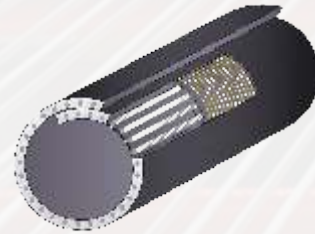
MAXX STEELFLEX™ MAXX ROUND® Pipe Belts with steel cord reinforcement
